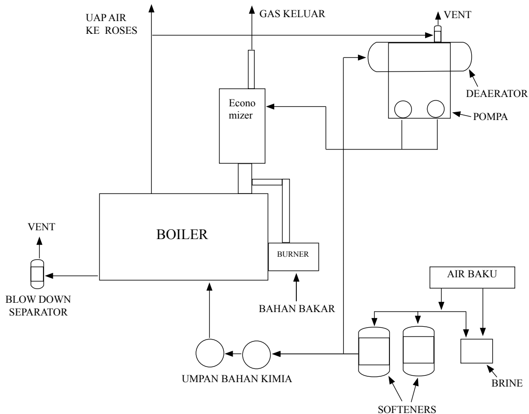
Gambar: Skema ruang boiler Referensi: National Productivity Council
