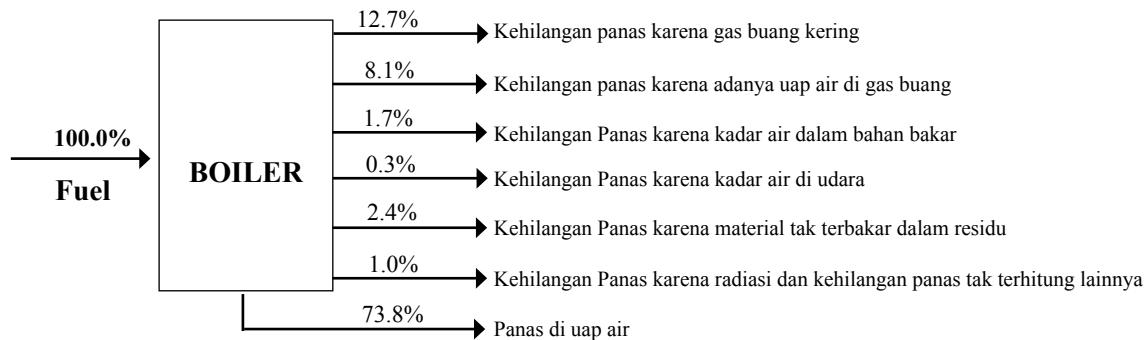
Gambar: Kerugian panas pada boiler berbahan bakar batubara ( coal fired boiler ) Referensi: National Productivity Council, Field Experience
