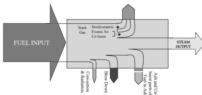
Gambar: Diagram neraca energi dari boiler Referensi: National Productivity Council, Field Experience
